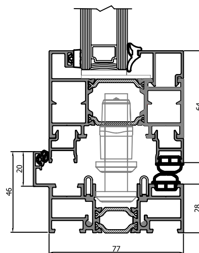
Bottom track 28 mm
