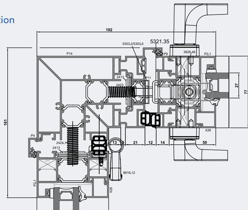
Section - Straight Edge Solution
