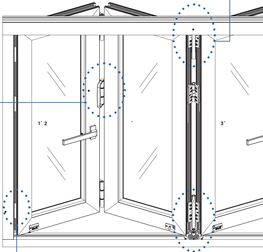
Art. 8816.14 Pulling hinge (external opening)
