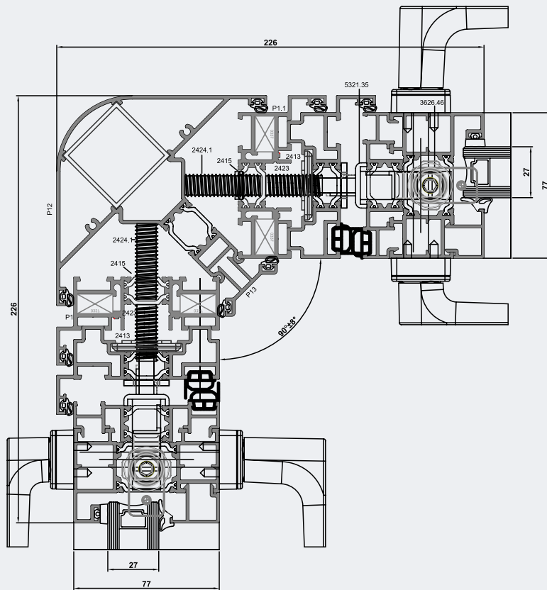
Section - Curved Corner Solution
