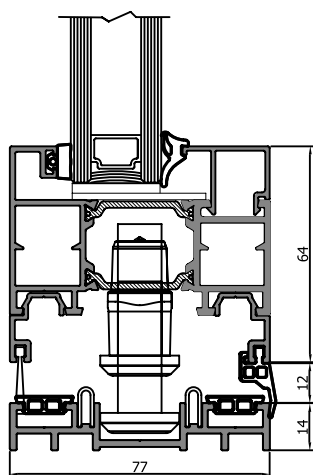
Bottom track 14 mm
